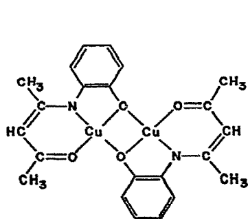
Fig. 1. Acetylacetone-mono( o -hydroxyanil)copper(II).
